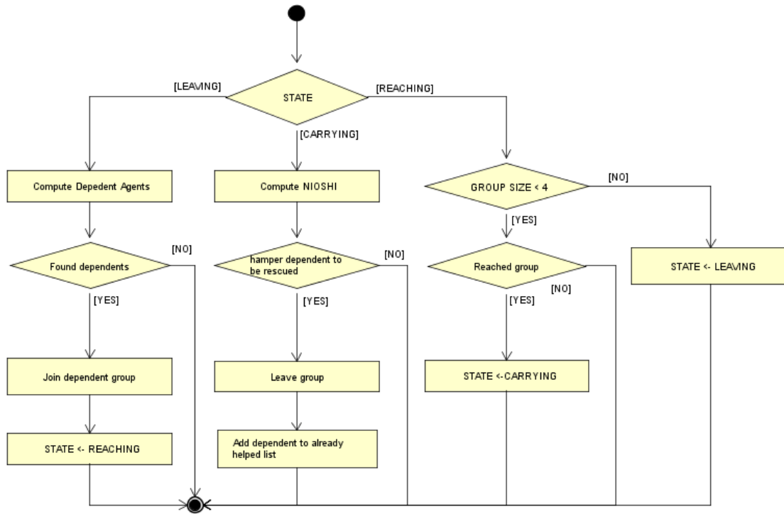
Figure 4: Flowchart of update execution.
