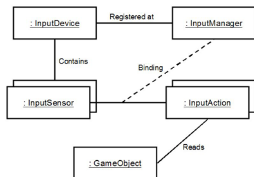
Figure 5 - Input System
