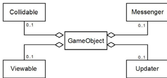
Figure 4: GameObject architecture
