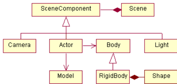
Figure 2: Scene and scene components classes.
