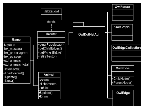
Figure 4: Class diagram
