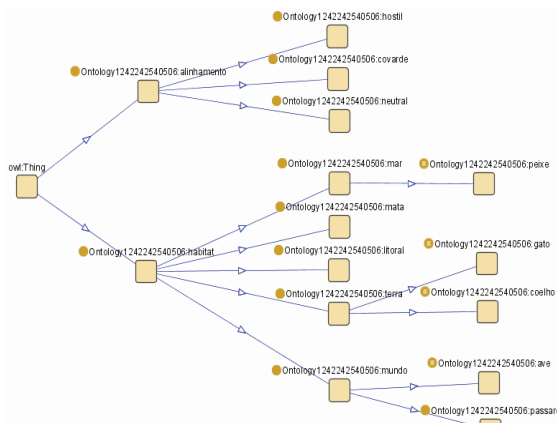
Figure 2: Ontology used in Ontological Trail
